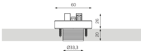
Cassaforma trimless rear - Rear trimless formwork (HOLEY_FRAME_TRLS_REAR)
