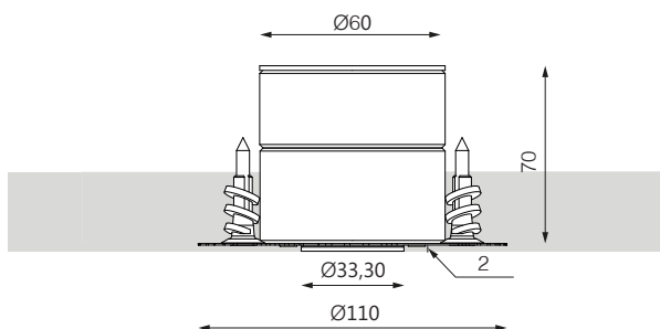
Cassaforma trimless - Trimless formwork (HOLEY_FRAME_TRLS_UL)
