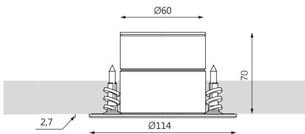
Cassaforma trim - Trim formwork (HOLEY_FRAME_REC_UL)
