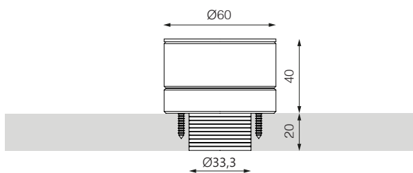
Cassaforma trimless rear - Rear trimless formwork (HOLEY_FRAME_TRLS_REAR_UL)
