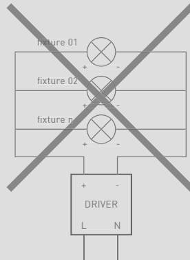
SEVERAL FIXTURES CONNECTION TO A SINGLE CONSTANT CURRENT DRIVER
