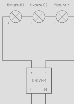
SEVERAL FIXTURES CONNECTION TO A SINGLE CONSTANT CURRENT DRIVER
